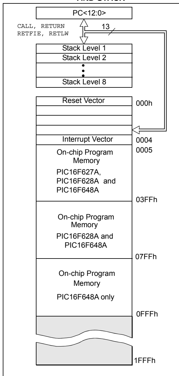
FIGURE 4-1: PROGRAM MEMORY MAP AND STACK
